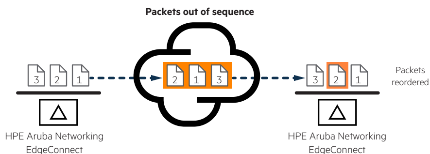
Figure 9. With Packet Order Correction, packets delivered out-of-order across the WAN are reordered into the correct
